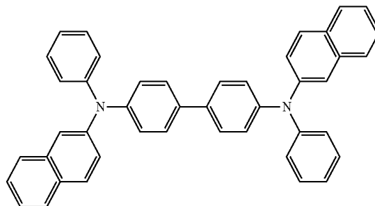
\beta -NPB
