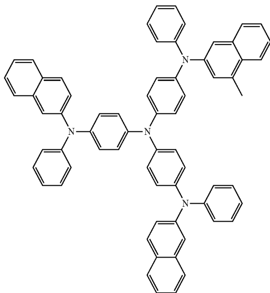
2-TNATA
