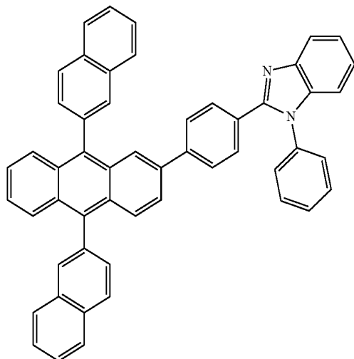
Chemical Formula 6-1
