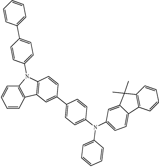
HT4
