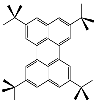
TBPc
