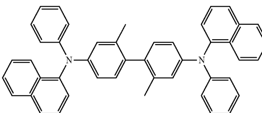
methylated NPB
